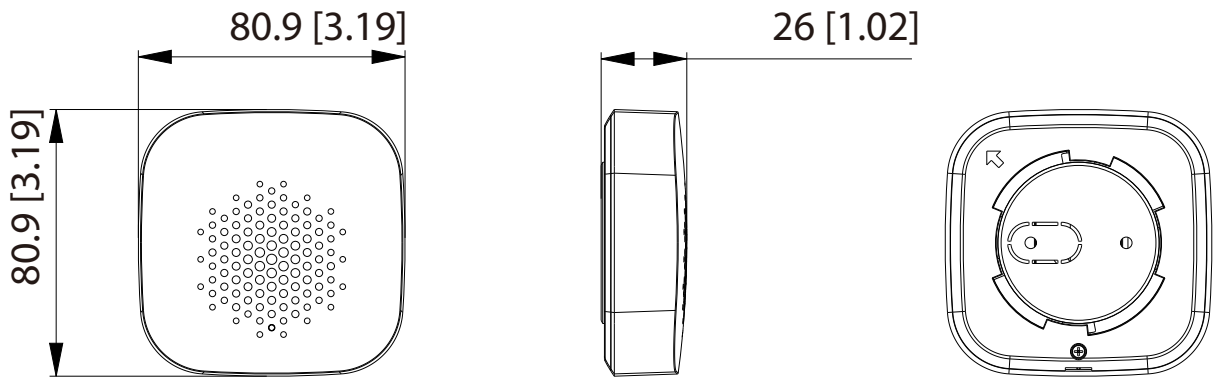
Figure 3-2 Dimensions (mm[inch])
