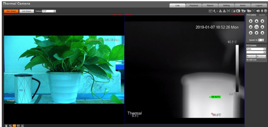
Figure 2-5 Live Interface
