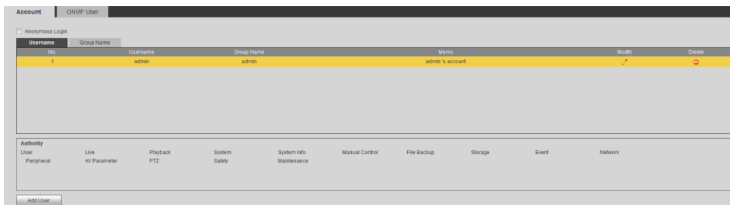
Figure 4-91 Username
