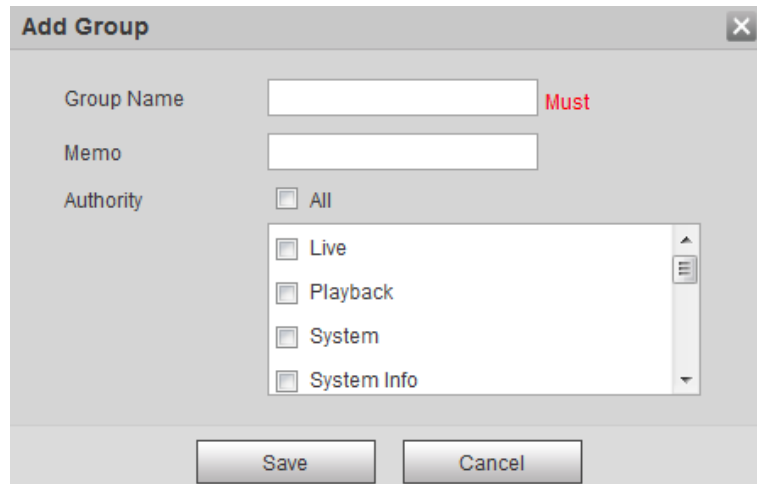
Figure 4-87 Add Group
