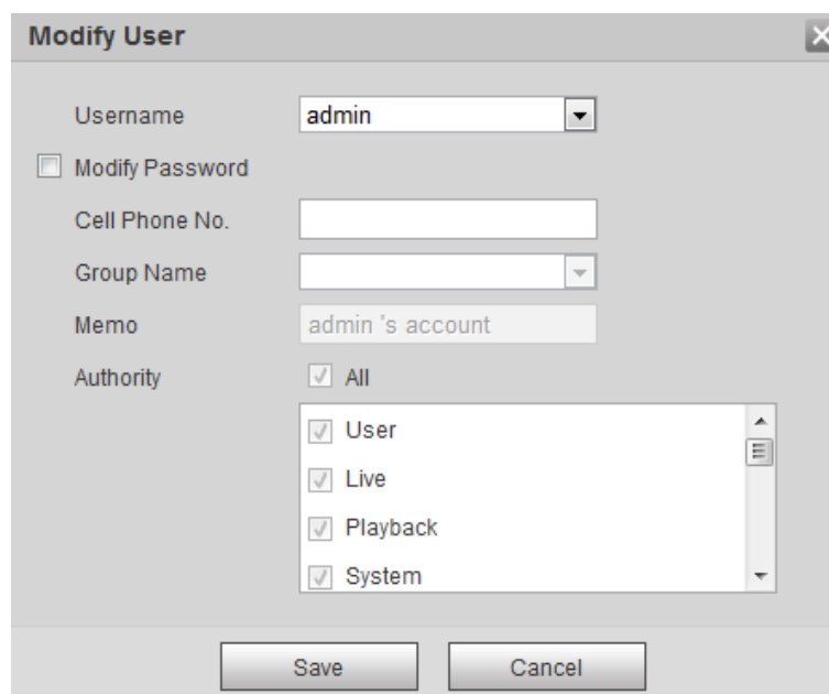
Figure 4-92 Modify user (1)
