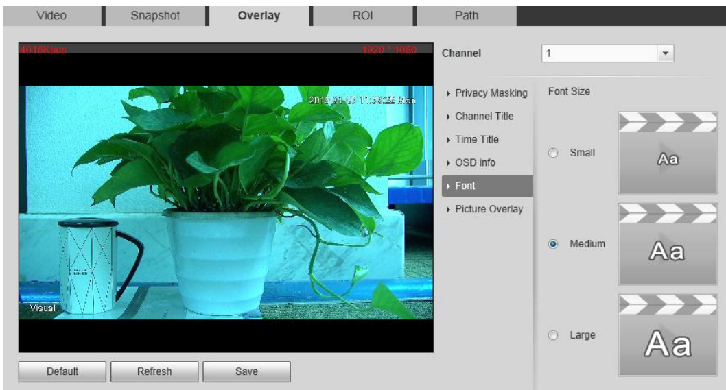
Figure 4-19 Font setting
