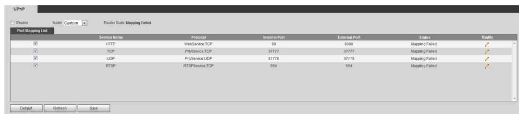
Figure 4-30 UPnP
