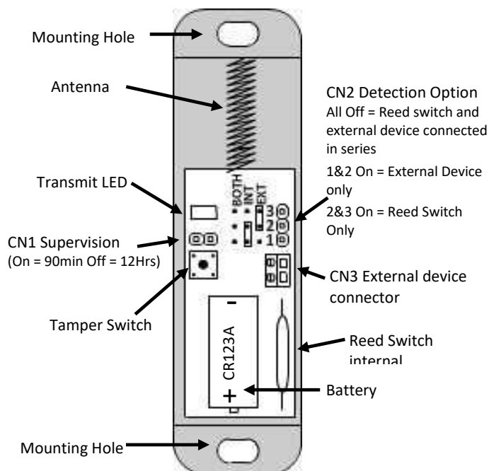
Figure 1: Wireless Door Mag
